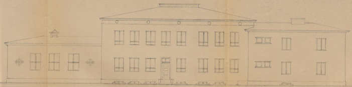
Tagantvaade (loodest)
